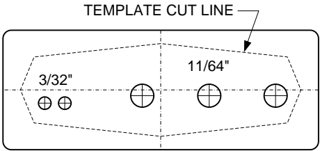
FRONT PANEL
