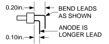
LED MOUNTING DETAIL
