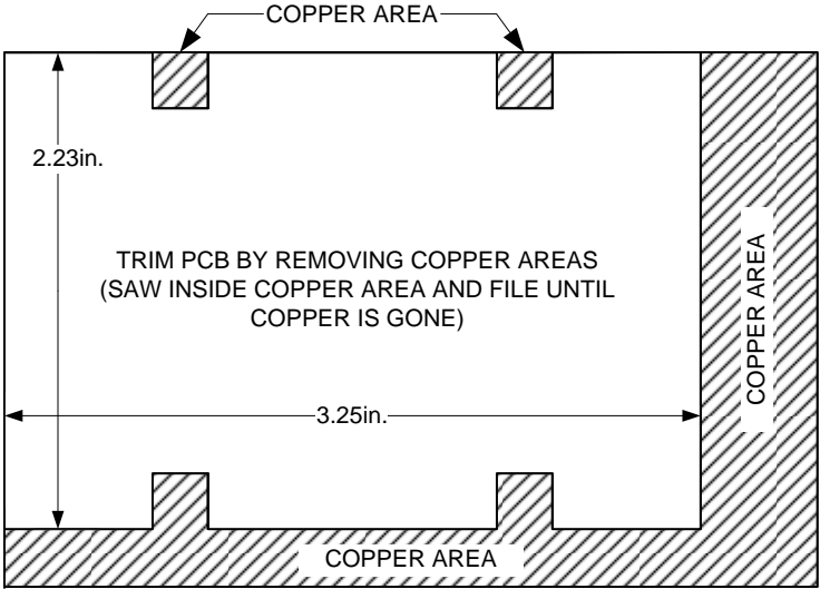
PC BOARD OUTLINE
