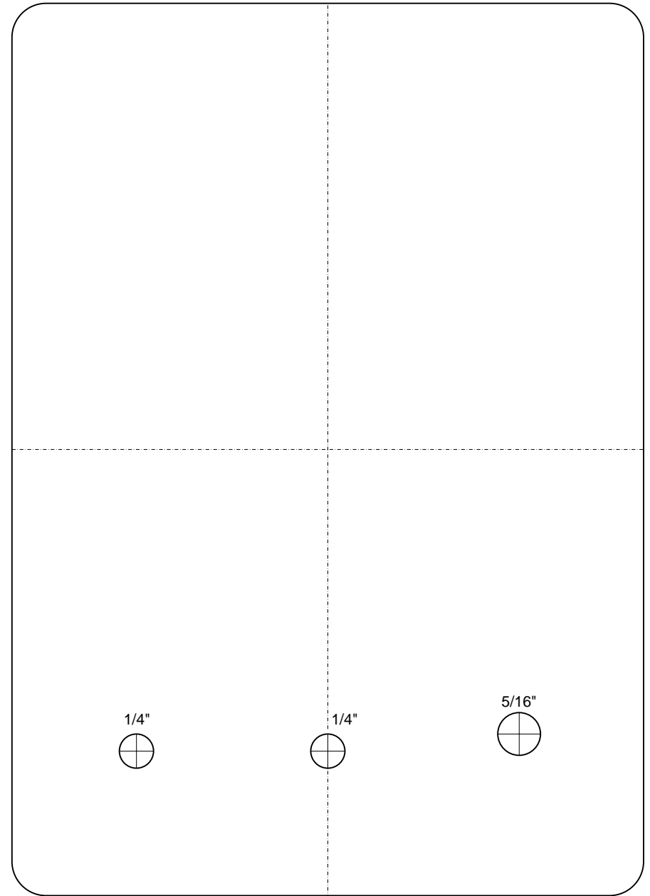
ENCLOSURE REAR
