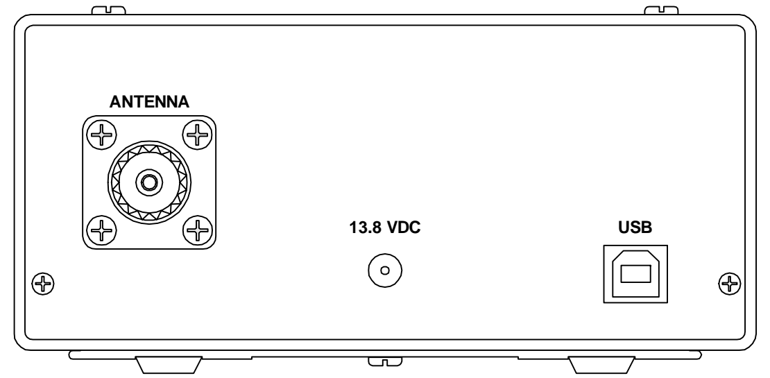
REAR VIEW
