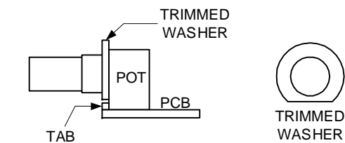
PC BOARD ASSEMBLY
