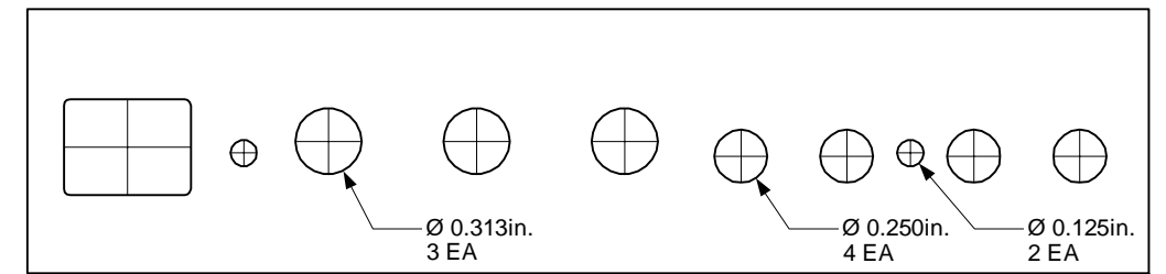
FRONT PANEL CUTOUTS
