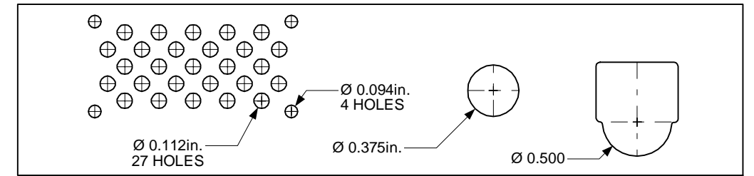
REAR PANEL CUTOUTS
