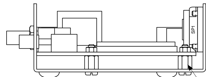
HEX MALE/FEMALE STANDOFF, 1/4" L X 4-40 THREAD, 4-40 X 1/4" L SCREW AND HEX NUT
