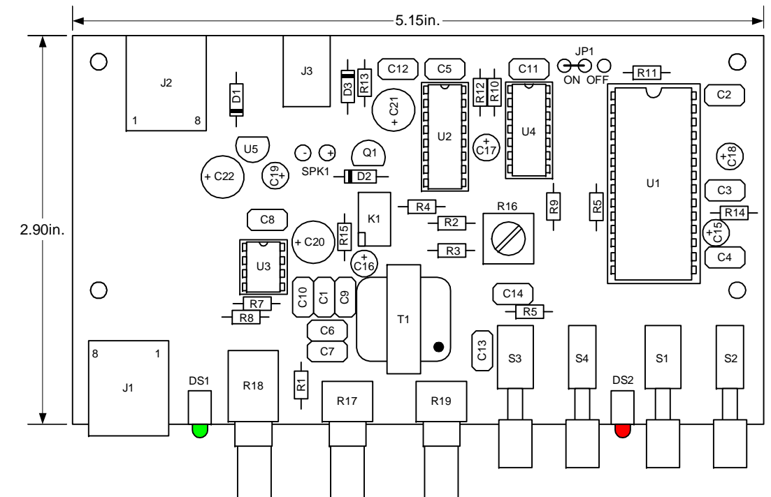
PC BOARD ASSEMBLY
