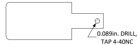
PADDLE CUTTING TEMPLATE MATERIAL: 1/8" COPPER PLATE, 2 EA
